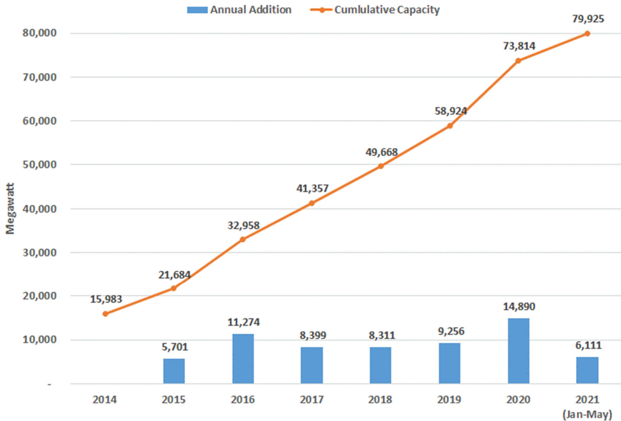
Figure 6-9: Installed U.S. PV capacity (Data source: EIA [4])
