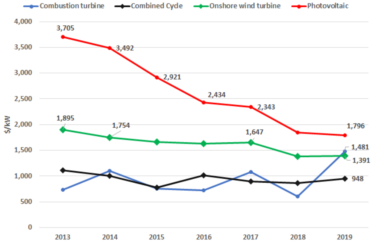
Figure 6-6: Average construction cost of generation installed in the U.S. 2013 to 2019 (Data Source: EIA [11])
