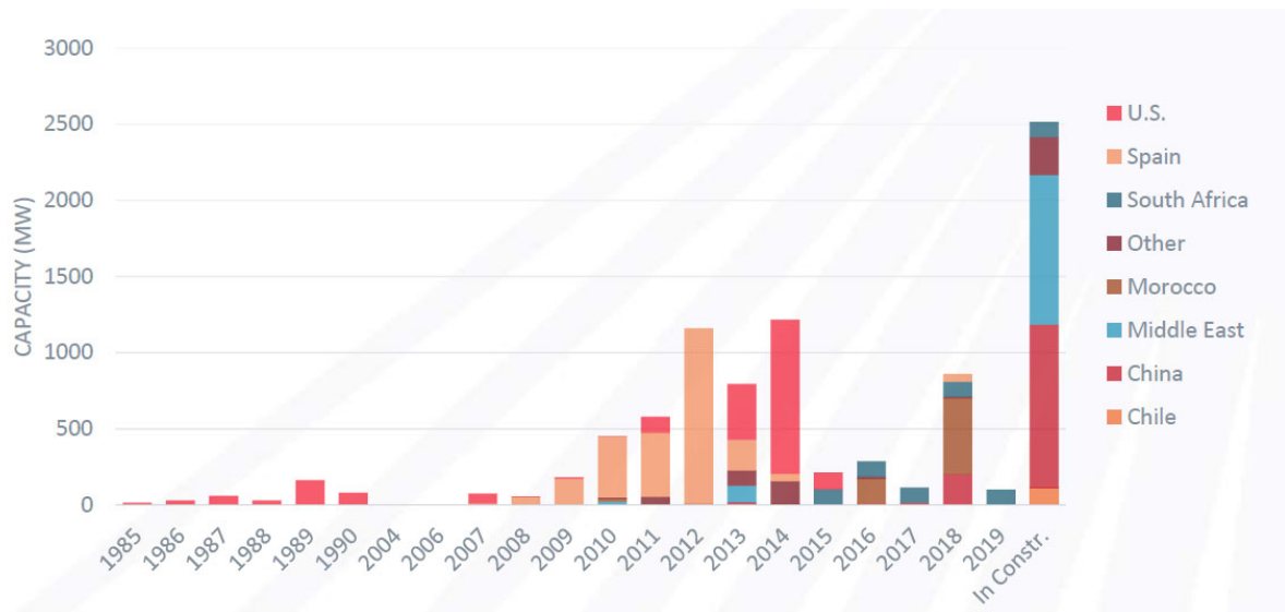
Figure 5-10: Solar thermal power capacity installation worldwide (Source: U.S. DOE [11])
