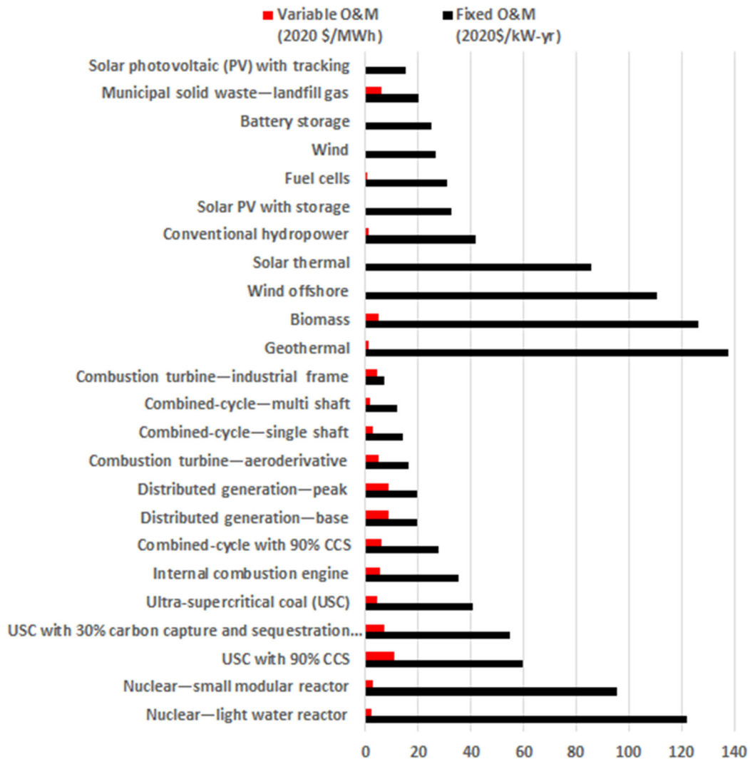
Figure 7-7: Estimated generating technologies fixed and variable O&M costs (Data source: EIA [13])
