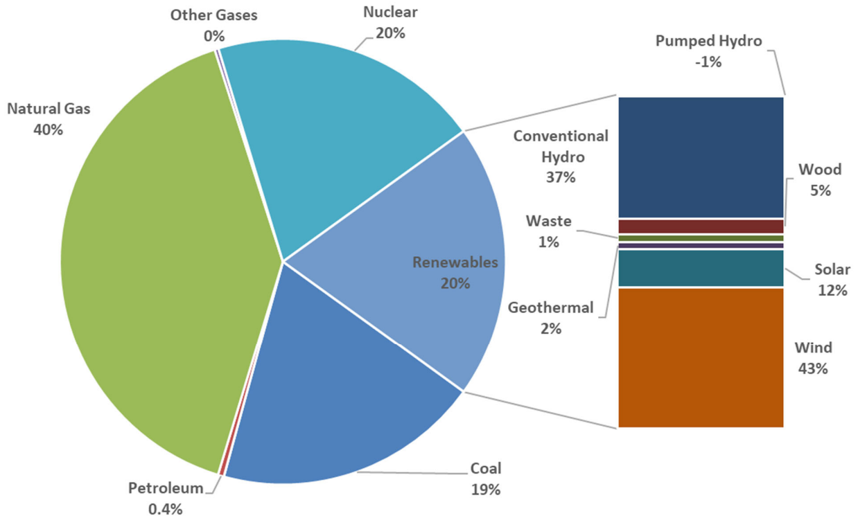
Figure 1-6: Net U.S. electricity generation by energy source in 2020 (Data source: EIA [6])
