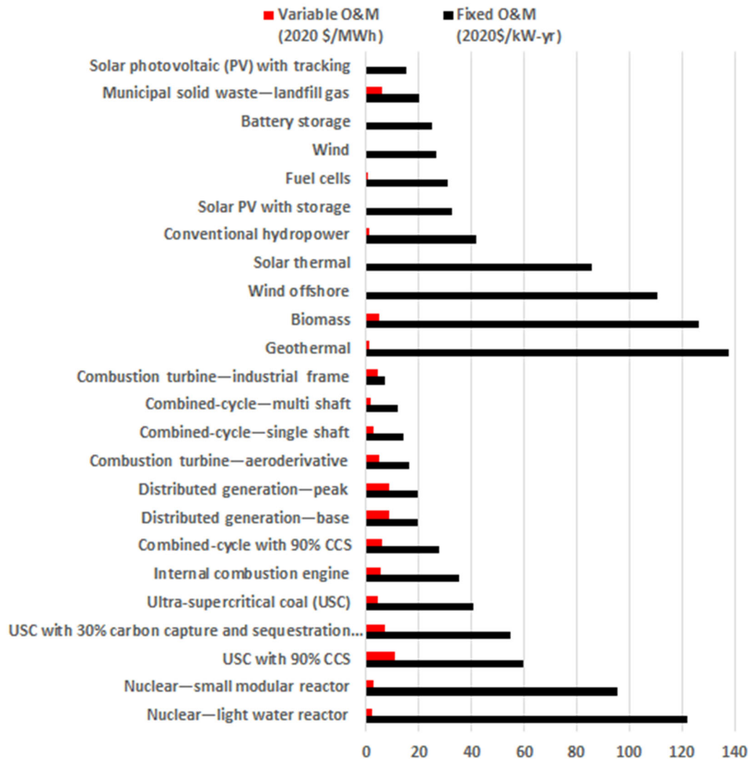
Figure 1-12: Estimated generating technologies fixed and variable O&M costs (Data source: EIA [17])
