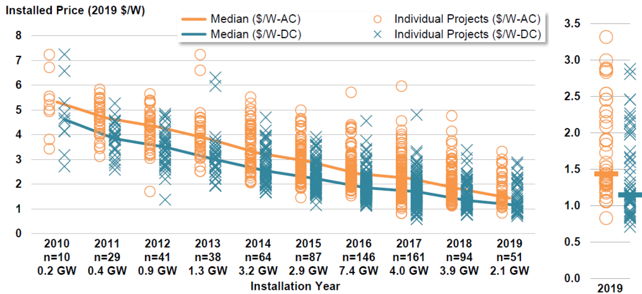
Figure 6-5: Installed price of utility-scale PV systems over time (Source: LBNL [10])
