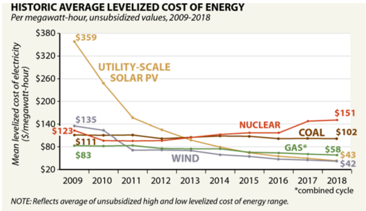
Figure 1-13: Historic average levelized cost of energy from various technologies (Source: InsideClimateNews using data from Lazard [18])
