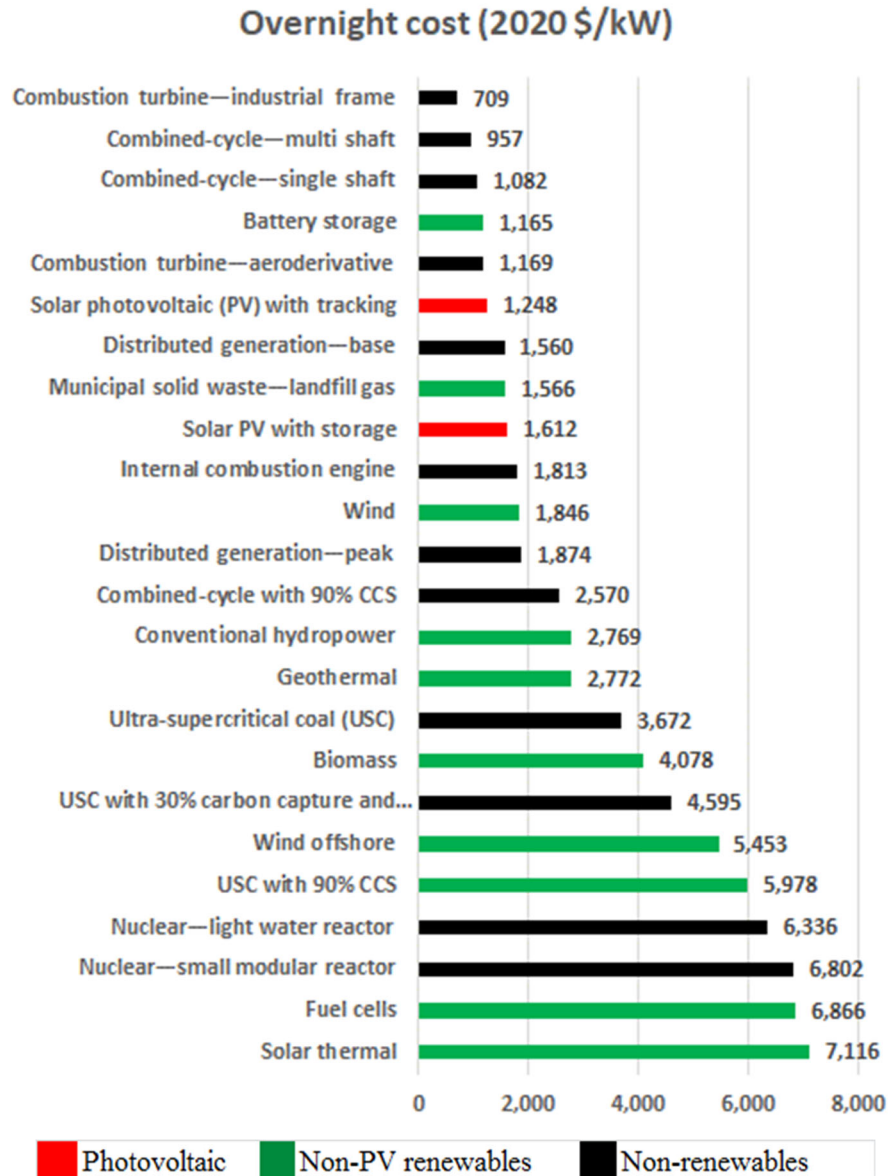
Figure 6-7: Estimated generating technologies capital costs (Data source: EIA [12])
