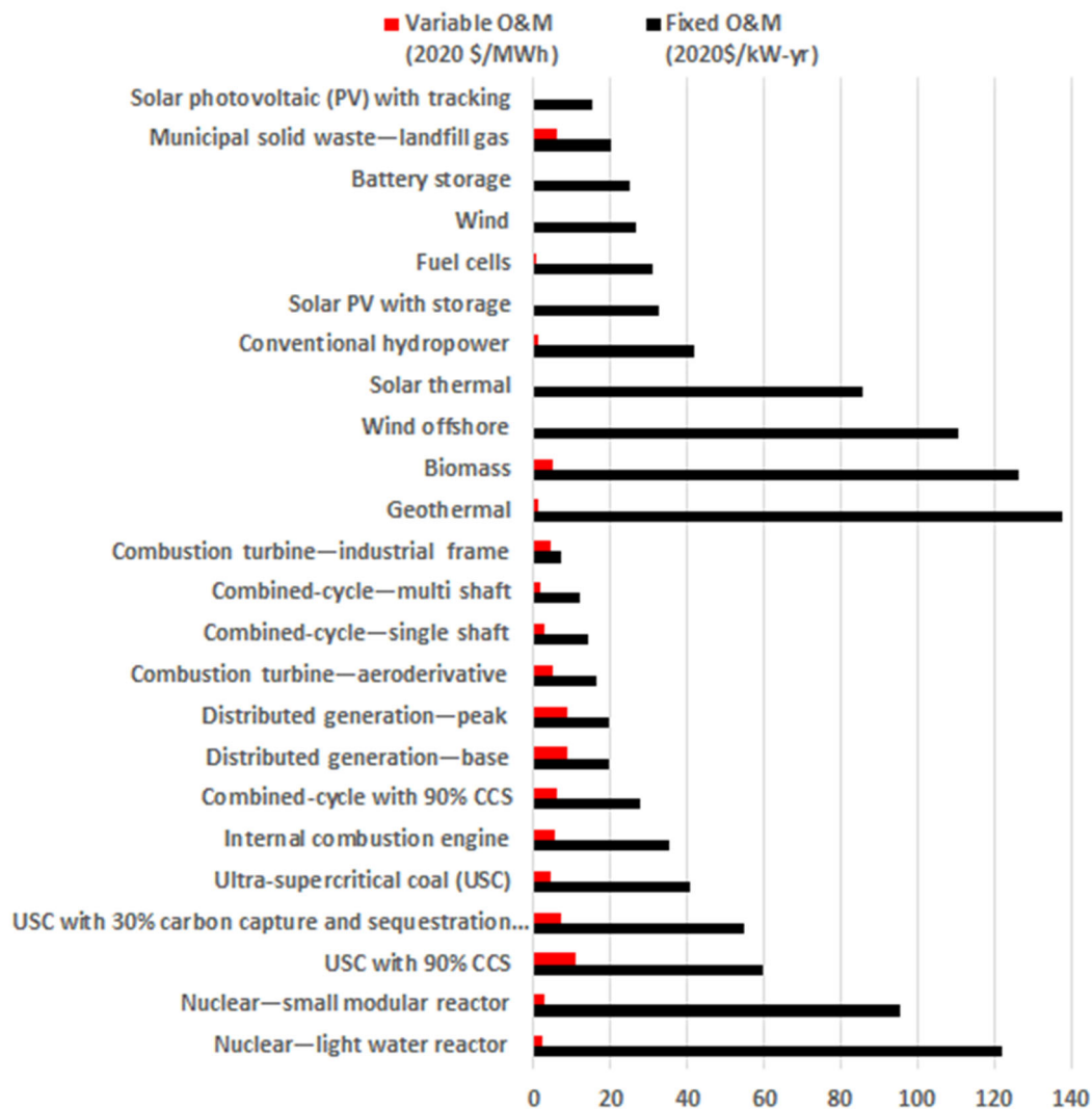
Figure 6-8: Estimated generating technologies fixed and variable O&M costs (Data source: EIA [12])
