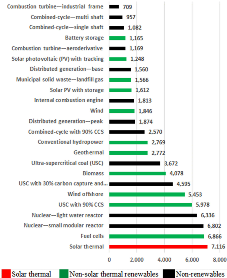
Figure 5-6: Estimated capital cost of generating technologies (Data source: EIA [6])
