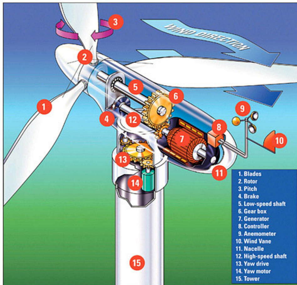
Figure 2-1: Horizontal wind turbine configuration (Source: Alternative Energy News [2])
