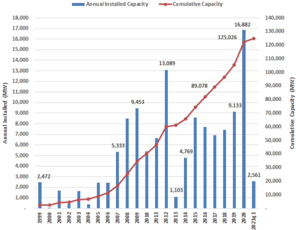
Figure 2-8: U.S. wind capacity growth (Sources: DOE [12], AWEA [13])
