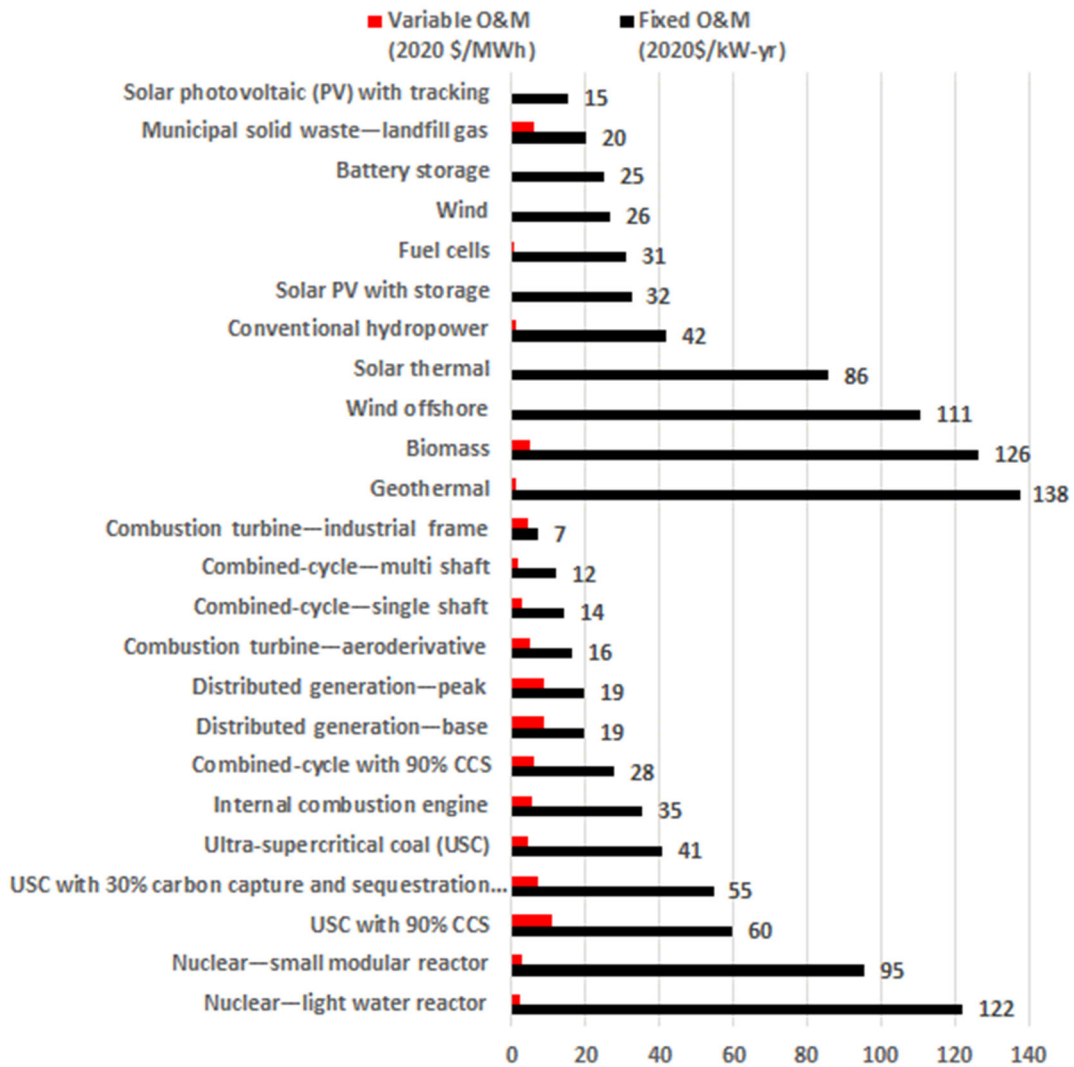
Figure 5-7: Operating and maintenance cost of generating technologies (Data source: EIA [6])
