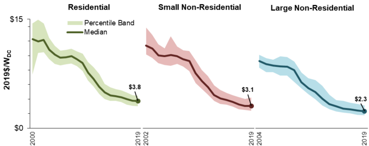
Figure 6-4: Installed price trends among grid-connected, distributed PV systems (Source: LBNL [9])
