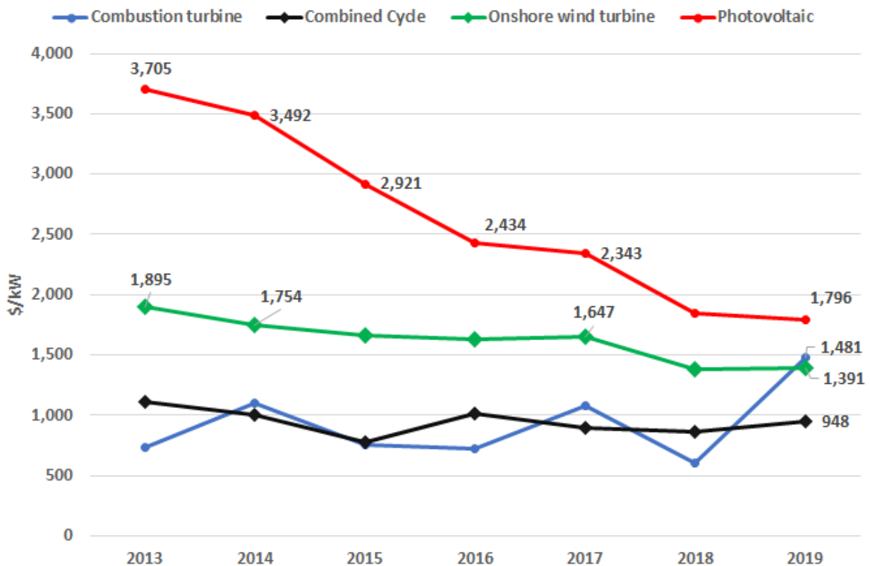
Figure 2-3: Average construction cost of generators installed 2013 to 2019 in the U.S. (Data source: EIA [9, 10])
