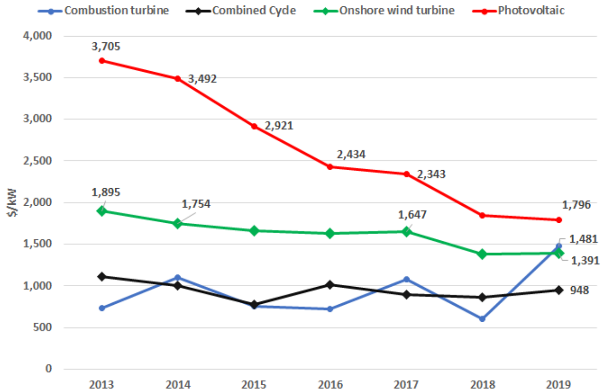
Figure 1-10: Average construction cost of generation installed 2013 to 2019 (Data source: EIA [16])
