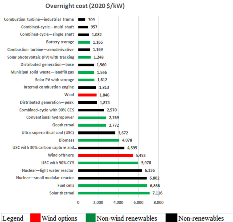
Figure 2-2: Estimated capital costs of various electric generation options (Data source: EIA [8])
