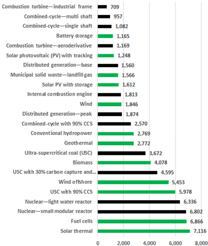
Figure 1-11: Estimated generating technologies capital costs (Data source: EIA [17])
