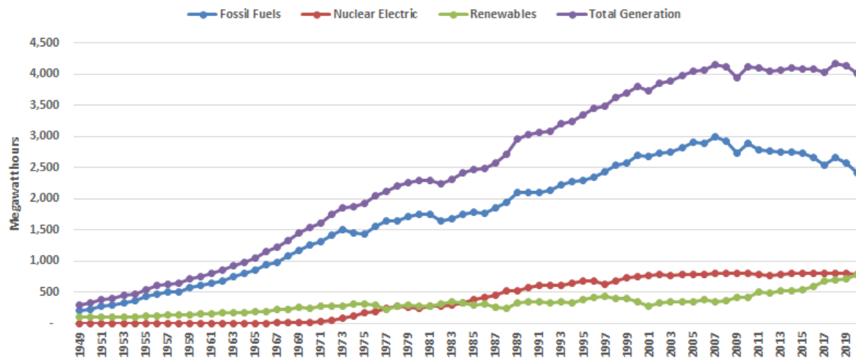
Figure 1-5: U.S. electricity generation by source (1949-2020) (Data source: EIA [6])
