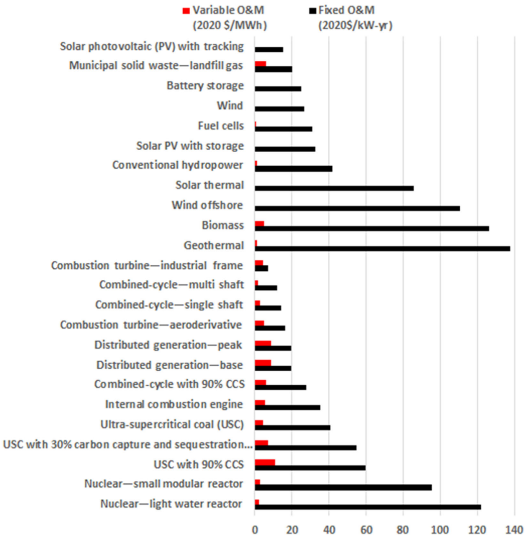
Figure 2-5: Estimated generating technologies fixed and variable O&M costs (Data source: EIA [8])
