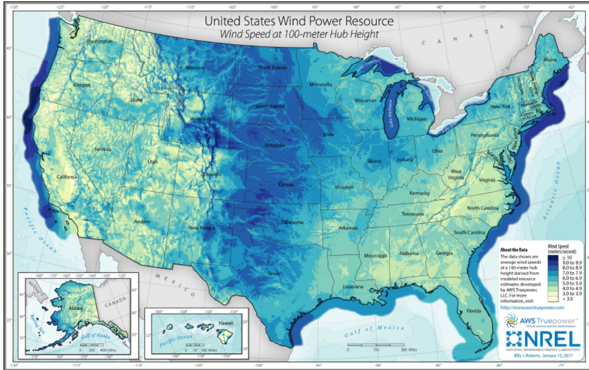
Figure 2-11: 100-meter U.S. wind resource map (Source: DOE [18])
