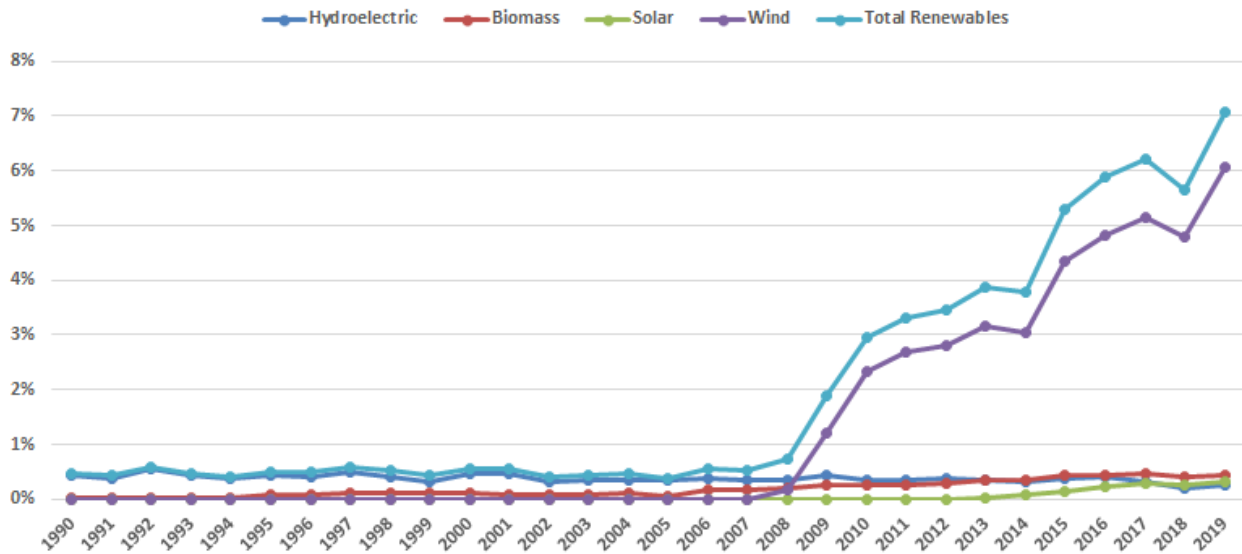
Figure 1-8: Renewables share of Indiana electricity generation (1990-2019) (Data source: EIA [8])
